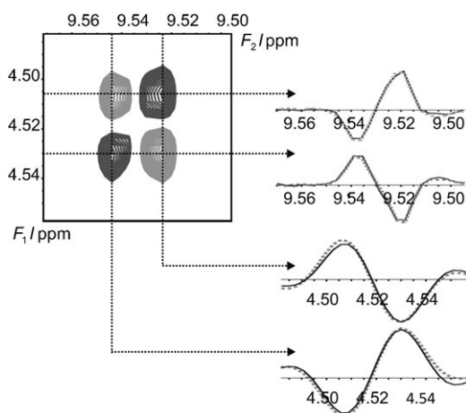
Figure 3. Fidelity of the lineshape reconstruction. The I13 HN-Ha peak from the IRLS-reconstructed DQF COSY spectrum of ubiquitin is shown. Positive contour levels are marked with dark gray, negative with light gray. 150 points (29.3%) were randomly selected from the full dataset (512 points). A sine-bell-weighted point distribution was used. The side panels show peak intersections (—) and a comparison with peak shape in the spectrum obtained with the full dataset (---).
